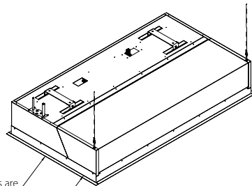
Suction grid with filter
