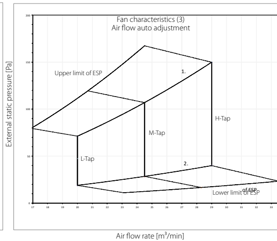
Air flow rate [m 3 /min]
